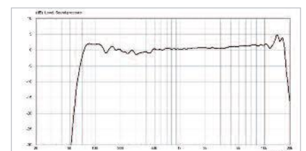
PS10-R2 response
